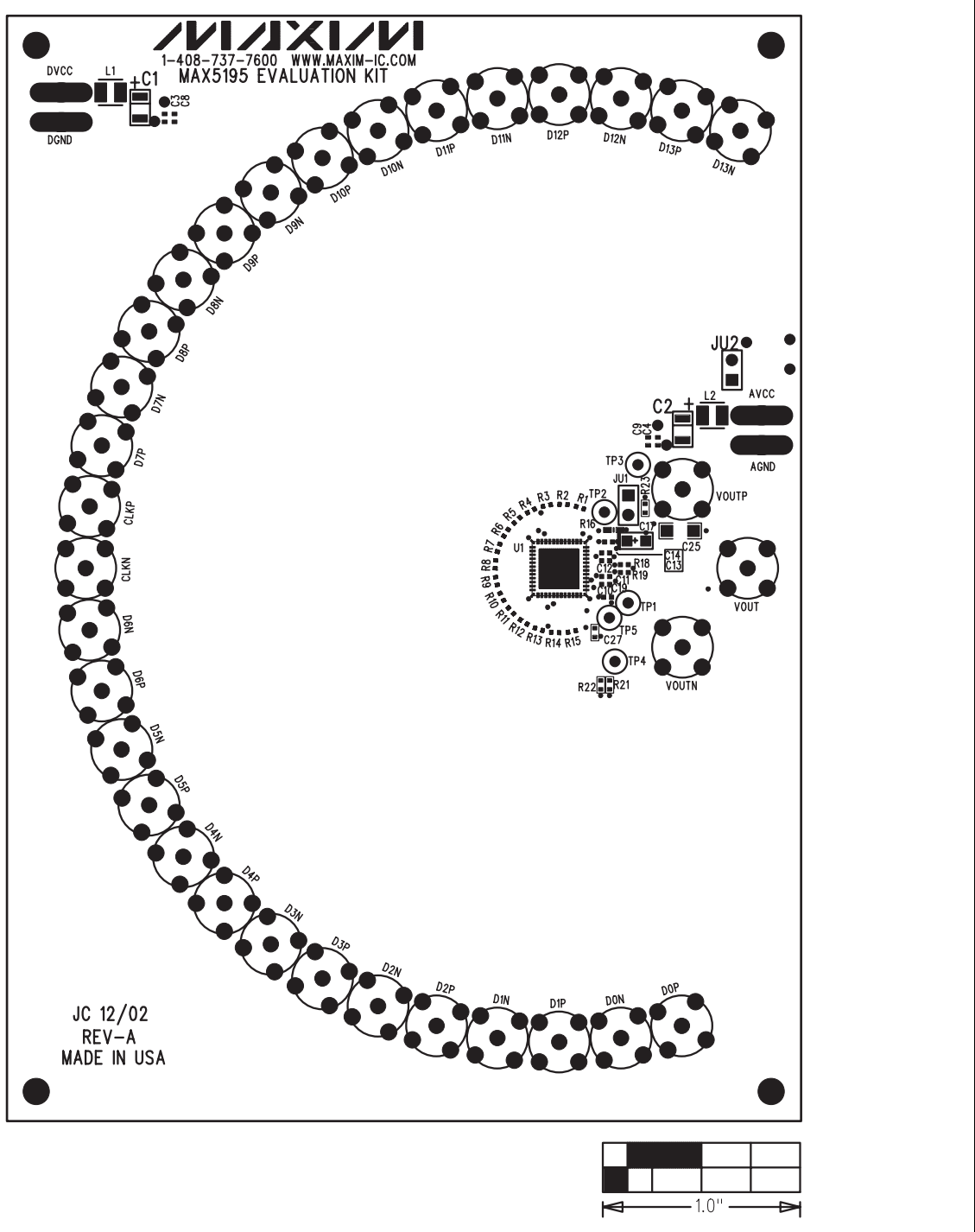
Figure 3. MAX5195 EV Kit Component Placement Guide—Component Side
